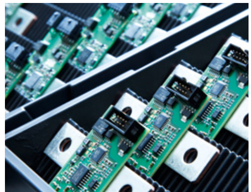
IVT-B sensor module on ESD rack prior to calibration
