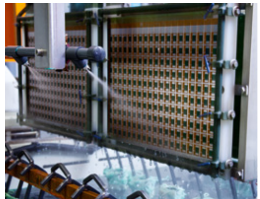
Plating process in new panel plating shop
