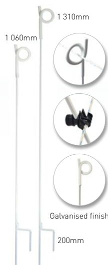
PIGTAIL STEEL POST (AA-PT/800W, AA-PT/1050W, AA-PT/800/G, AA-PT/1050/G)
