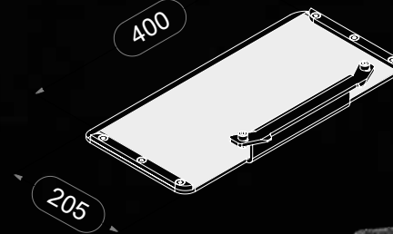
Toe plate to hook on for crates with drinks 400 x 205 mm
