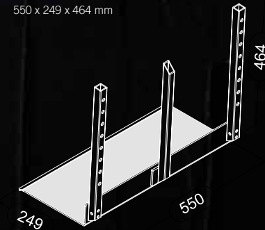
25 cm - regular beams 550 x 249 x 464 mm
