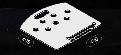
Toe plate to hook on 430 x 405 mm
