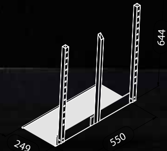
25 cm - extended beams 550 x 249 x 644 mm
