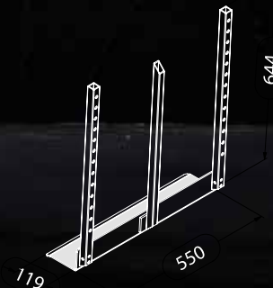
Standard 12 cm - extended beams 550 x 119 x 644 mm
