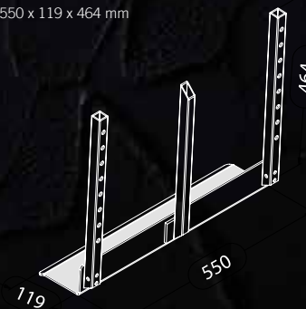
Standard 12 cm - regular beams 550 x 119 x 464 mm
